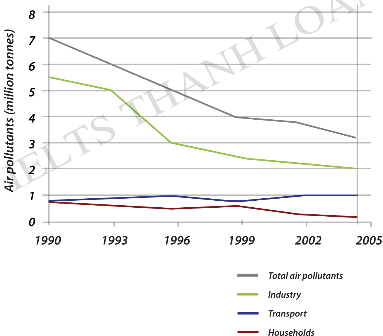
Sources of UK air pollutants (million tonnes), 1990 - 2005
